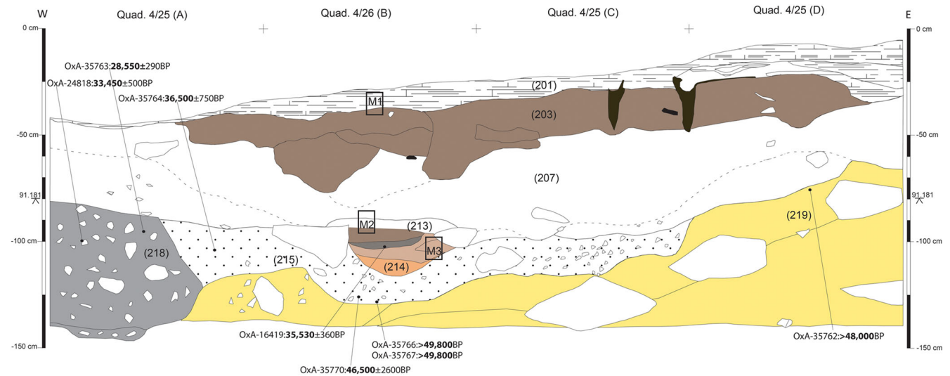
Figure 5. A representative west–east stratigraphic section at TT with the location of micromorphological samples. [Color figure can be viewed at wileyonlinelibrary.com]
